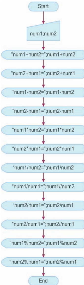
Flowchart of the Program "05calculator"
