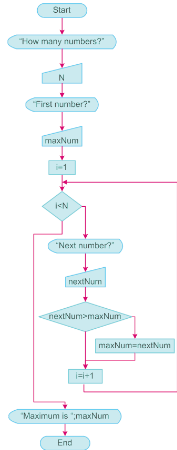
Flowchart of the Program "max"
