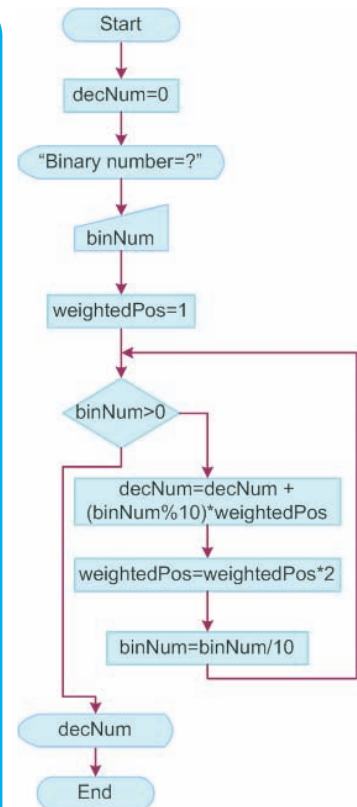
Flowchart of the Program "bintodec"
